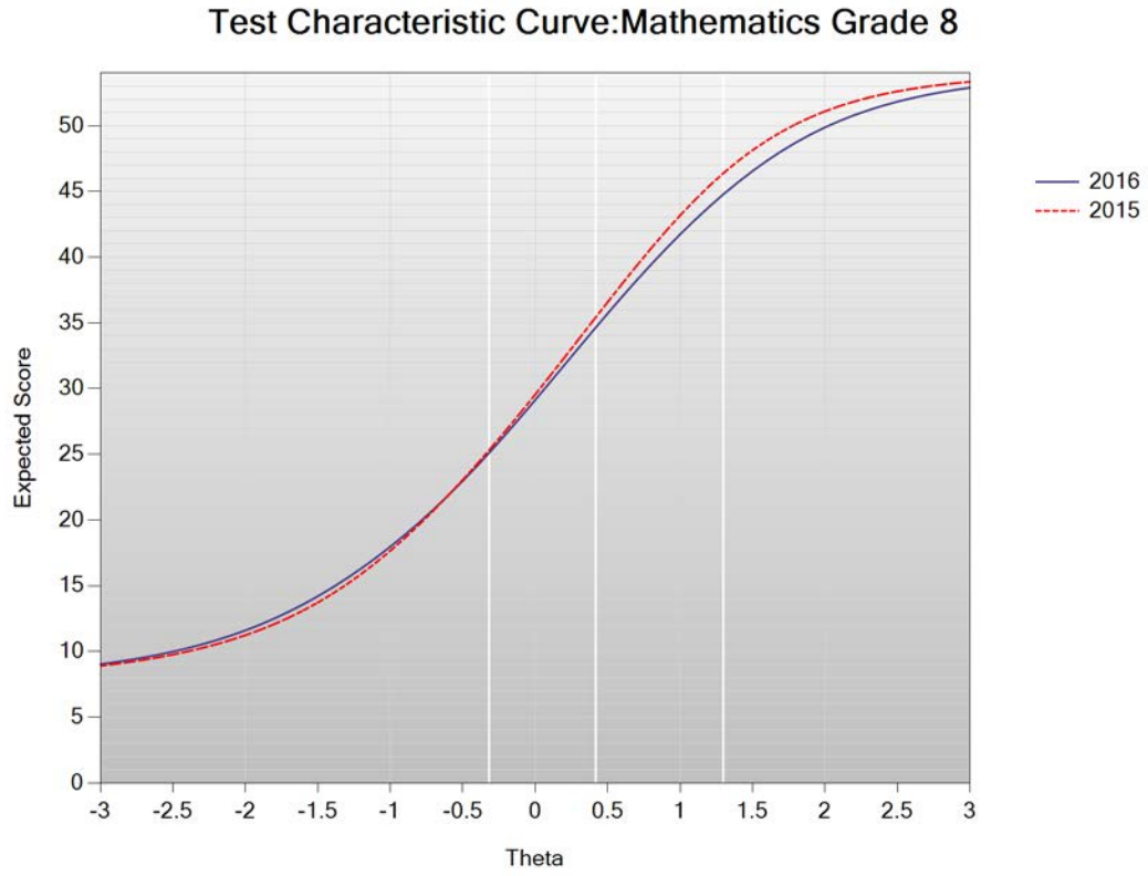
Figure I-25. 2016 MCAS: Test Characteristic Curve – Mathematics Grade 8
