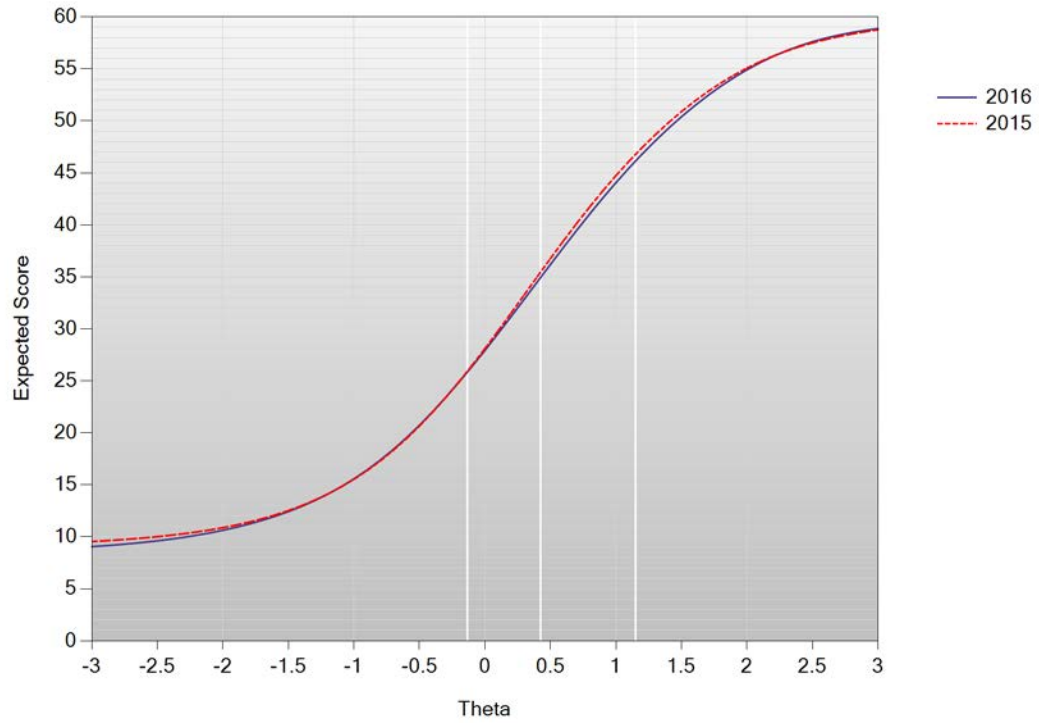
Test Characteristic Curve: Chemistry Grade 10
