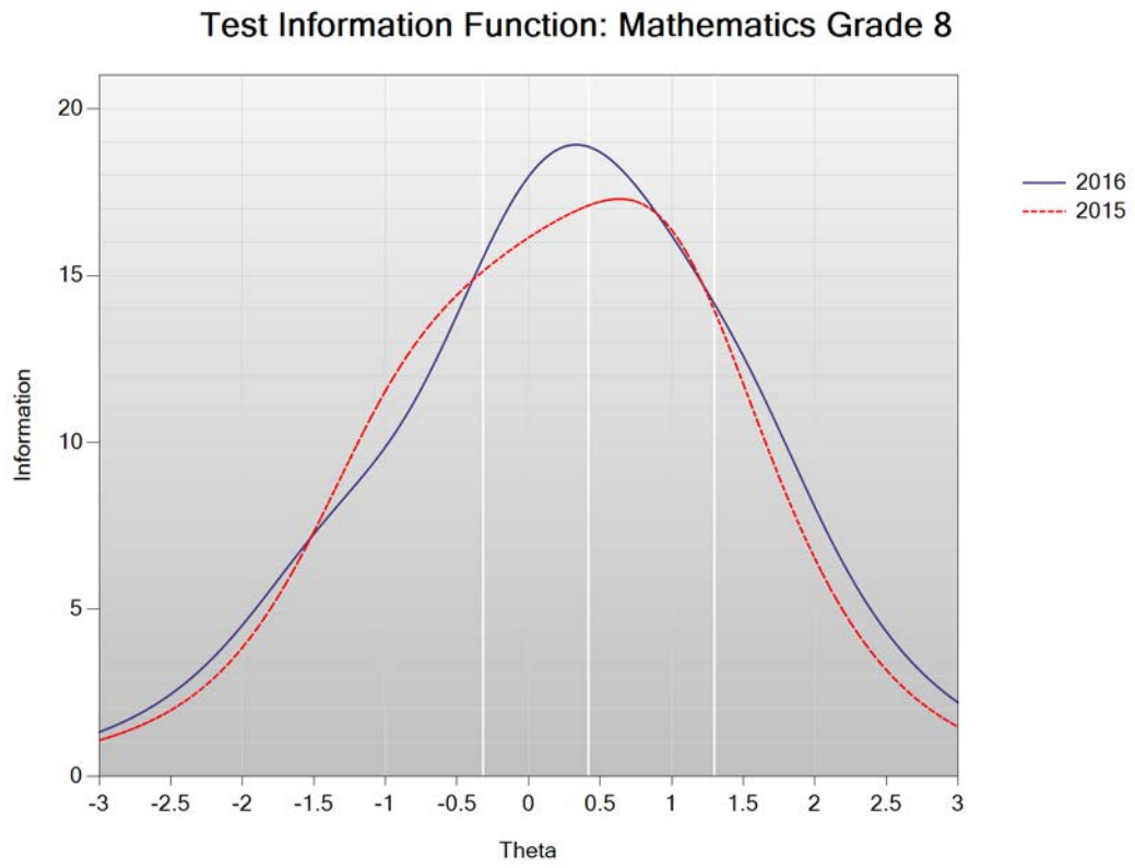
Figure I-26. 2016 MCAS: Test Information Function – Mathematics Grade 8
