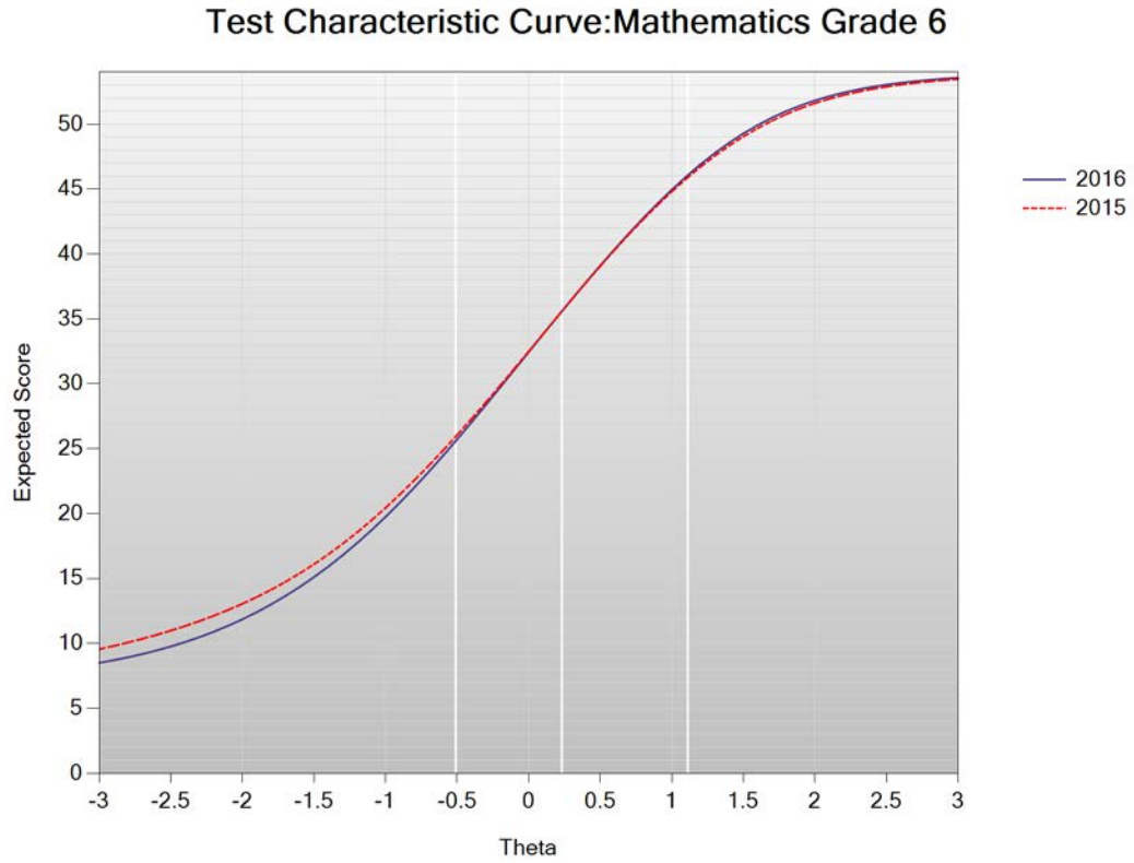
Figure I-21. 2016 MCAS: Test Characteristic Curve – Mathematics Grade 6
