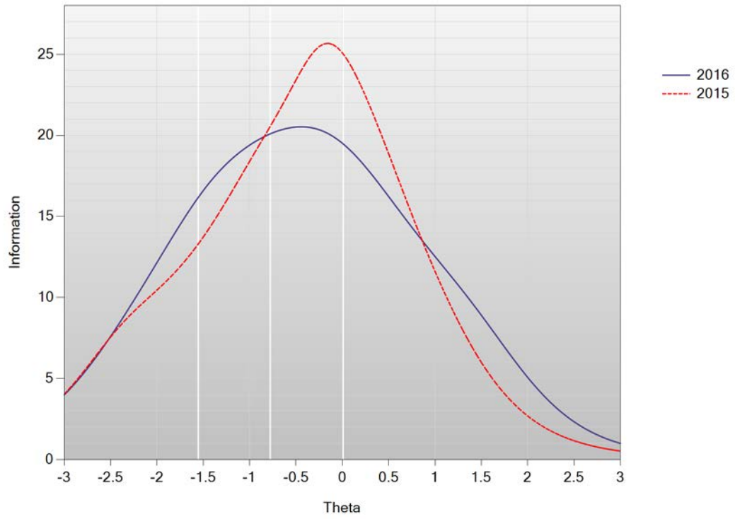
Test Information Function: Mathematics Grade 10
