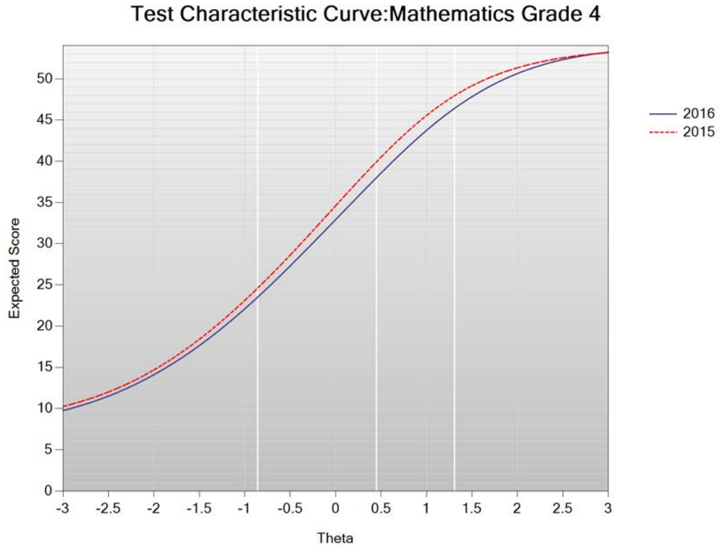
Figure I-17. 2016 MCAS: Test Characteristic Curve – Mathematics Grade 4
