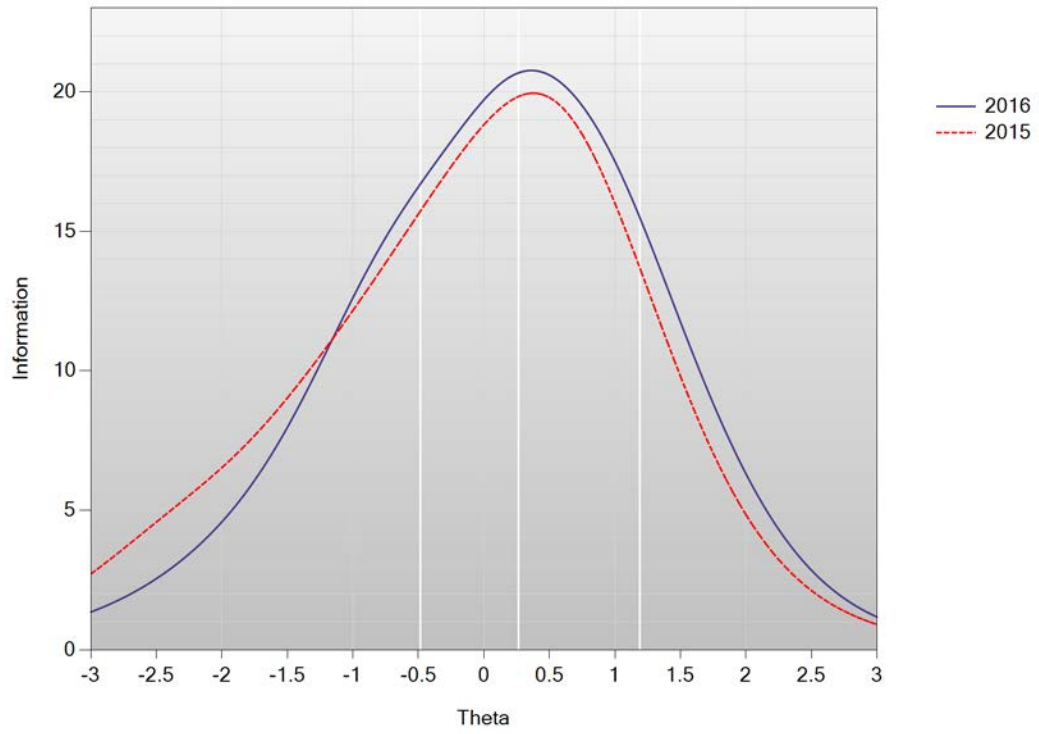
Test Information Function: Mathematics Grade 7
