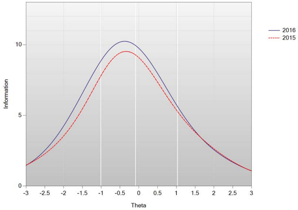
Test Information Function: Mathematics Grade 3
