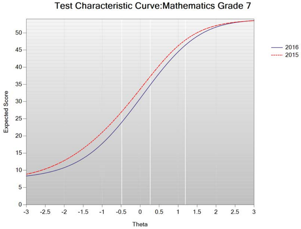
Figure I-23. 2016 MCAS: Test Characteristic Curve – Mathematics Grade 7
